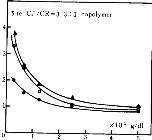
Fig. 2. Reduced viscosity of polymer solution. (▲: K^+/CR=3 , ○: C_s^+/CR=3 , ●: R_b^+/CR=3 ) (Ref. Han (1984))
