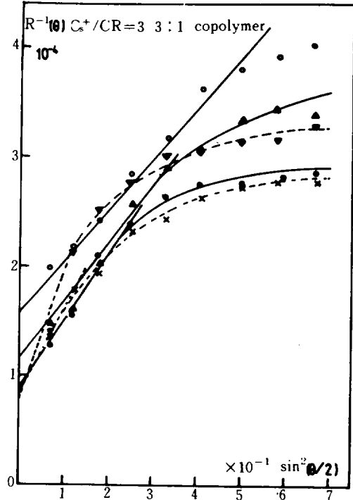
Fig. 3. R^{-1}(\theta) as a function of \sin^2(\theta/2) for solution 3:1 copolymer with C_s^+/CR=3 . (○; C=0.05g/dl , ▲; c=0.025g/dl , ▲; c=0.0125g/dl , ●; c=0.003125g/dl )
