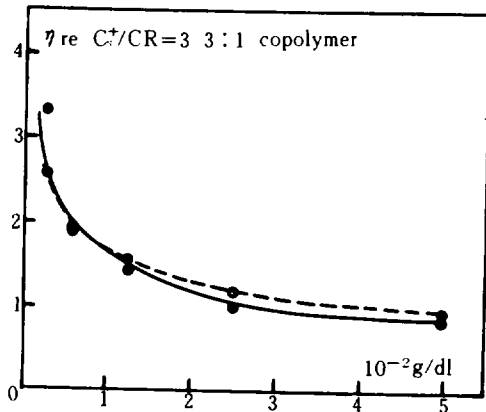
Fig. 5. Reduced viscosity calculated from light scattering data (dashed line) and measured with a viscometer (solid line) for solution of 3:1 copolymer ( C_s^+/CR=3 ).
