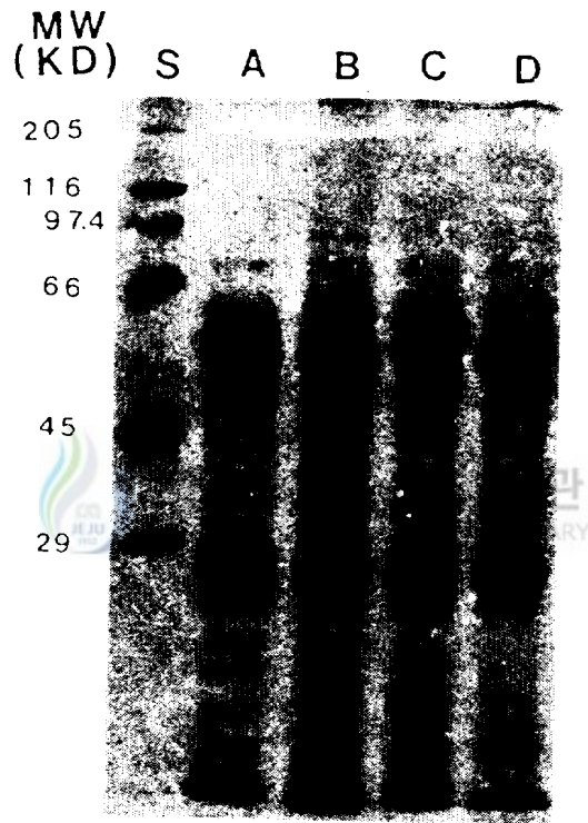
Fig.1. Protein banding patterns of Goodyera by SDS PAGE.
