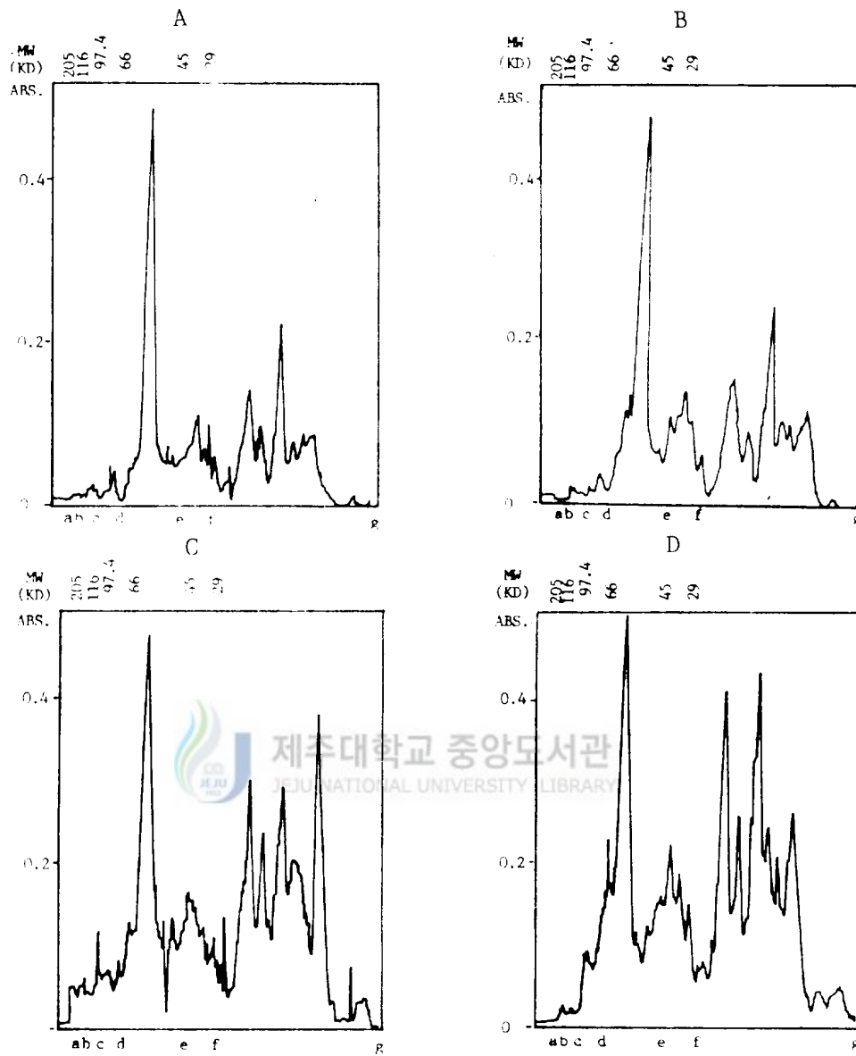
Fig.2. Densitometric recordings of the electrophoretic pattern of proteins in Goodyera .
