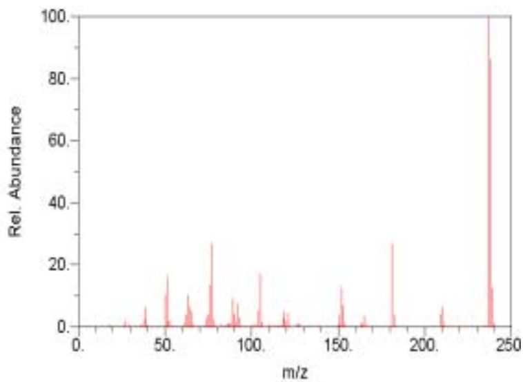
Fig. 3. Mass analytic spectrum of dihydro-flavonol separated from hypofracted fluid.
