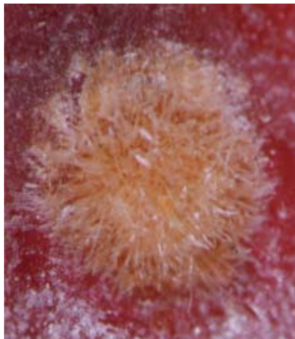
Figure 2. Shape of spine in Opuntia ficus-indica var. Saboten
