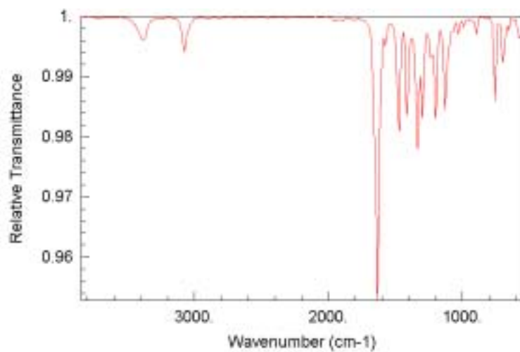
Fig. 5. IR spectrum of dihydro-flavonol separated from hypofracted fluid.
