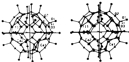
Fig. 2. A stereoview of the sodalite unit of dehydrated \text{Ca}_{5.6}\text{Tl}_{0.4}\text{-A} . Another about 40% of the sodalite units have this arrangement. Ellipsoids of 20% probability are used.
