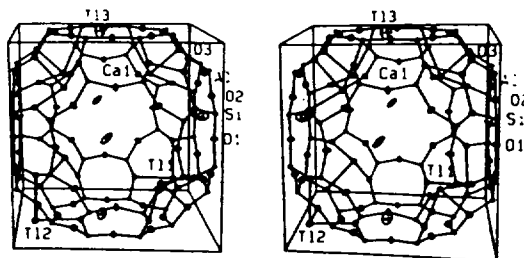
Fig. 4. A stereoview of the large cavity of dehydrated \text{Ca}_{14}\text{Tl}_{9.2}\text{-A} is shown using ellipsoids of 20% probability.
