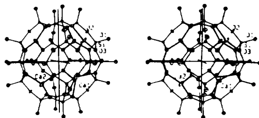
Fig. 1. A stereoview of the sodalite unit of dehydrated \text{Ca}_{5.6}\text{Tl}_{0.4}\text{-A} . About 40% of the sodalite units have this arrangement. Ellipsoids of 20% probability are used.
