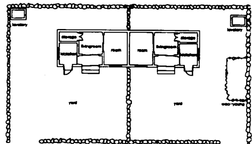
Fig. 2 Floor plan of Urban Type House for The sufferers(Located at Bong-gae, 1959)
