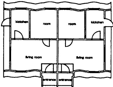
Fig. 12 Sam-an type House for Two Generation (Located at Isidol a pasture)
