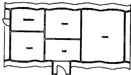
Fig. 11 Sam-an type House for One Generation (Located at Isidol a pasture)
