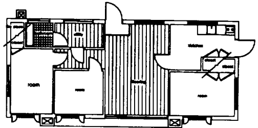
Fig. 4 Floor plan of Welfare House (Located at Samdo-1dong)
