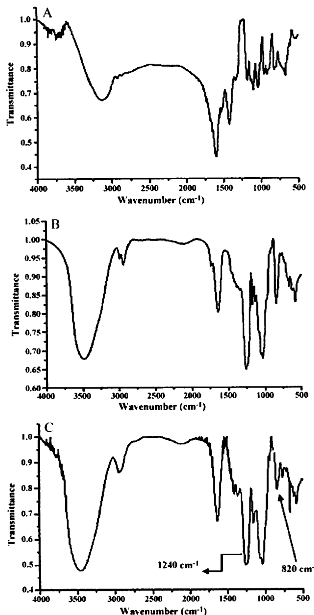
Fig. 2. FT-IR frequencies of bands for (A) crude polysaccharide fraction, (B) purified ECSP and (C) commercial fucoidan.
