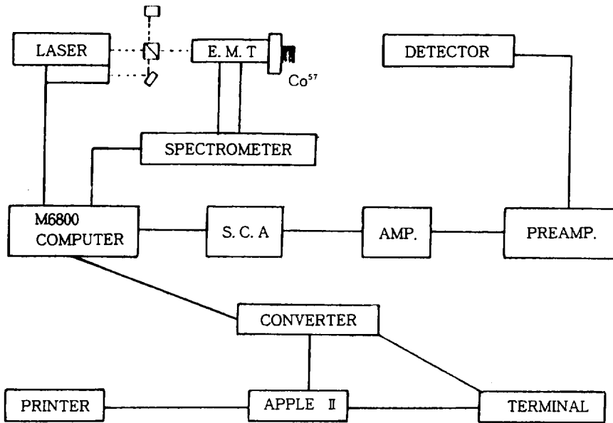
Fig. 1. Block diagram of Mössbauer spectrometer.
